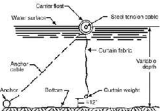
TYPICAL FLOTATION SILT CURTAIN NOT TO SCALE
