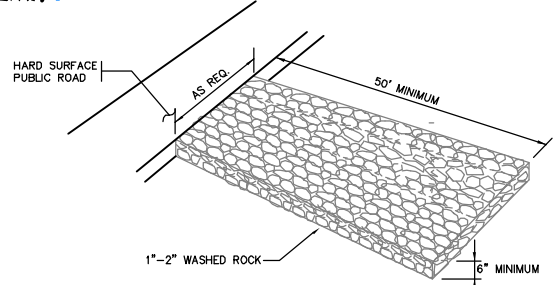
TYPICAL ROCK SURFACE (INSTALLED) NOT TO SCALE
